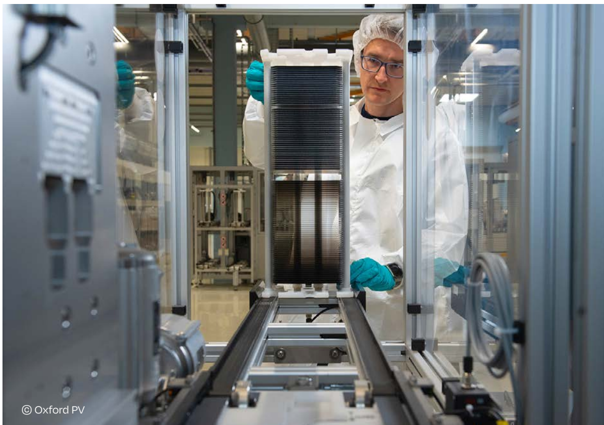
Oxford PV integrated cell production line in Brandenburg, Germany
