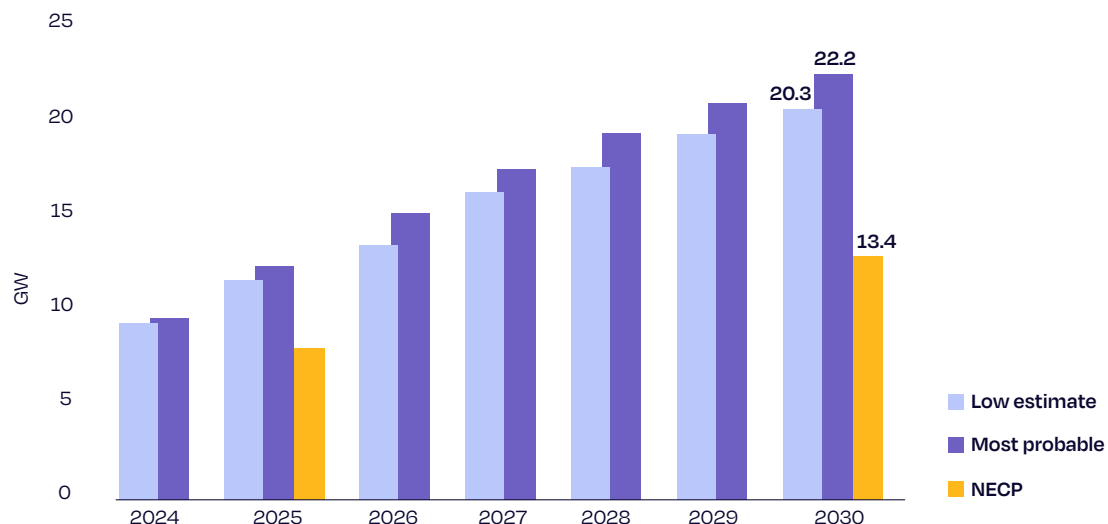
Cumulative solar PV capacity scenarios 2024-2030
